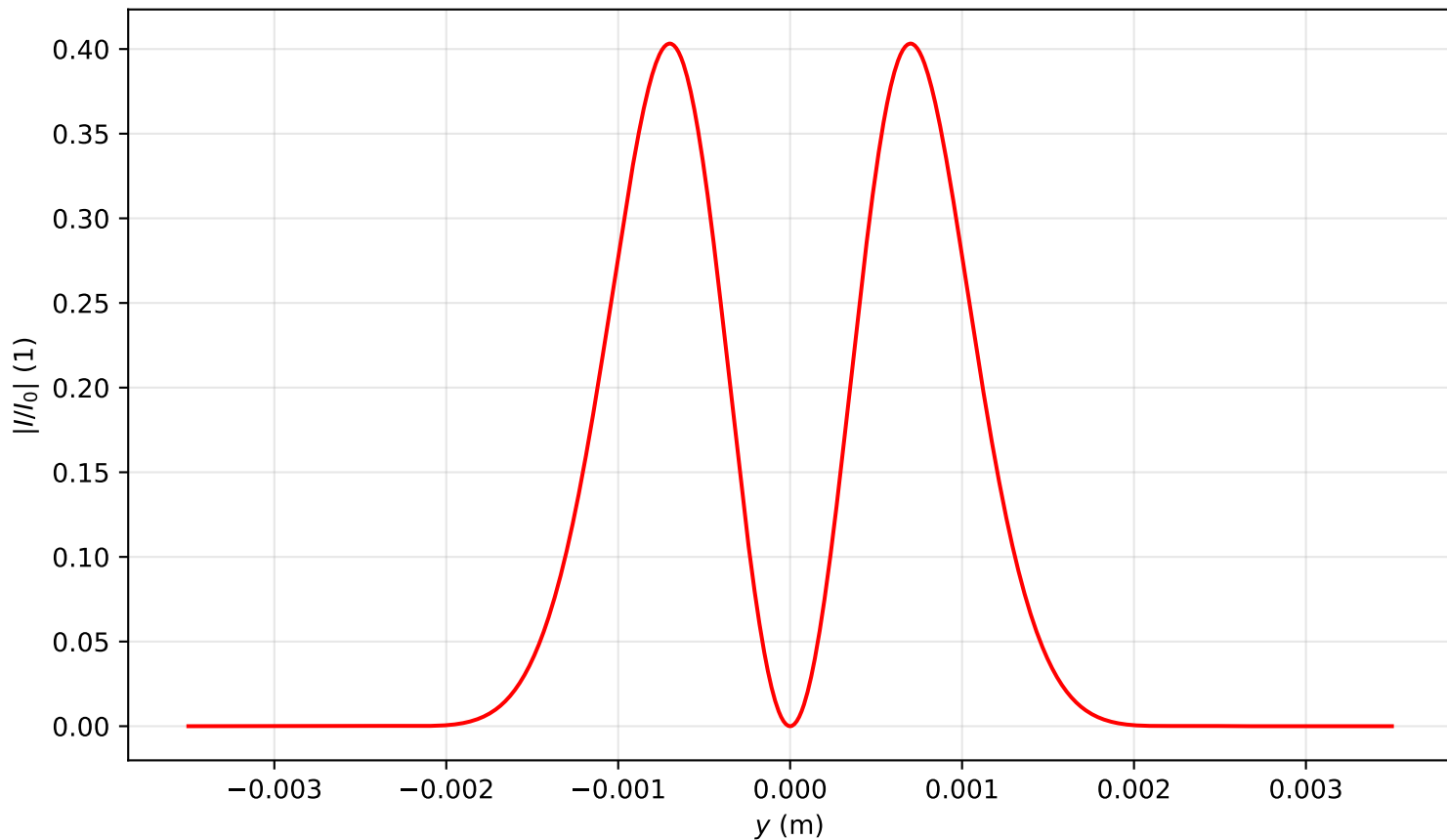
Intensity profile I(x=0, y, z=2.070)/I_0 , P_{in}=1.0P_{cr} , artificial time
